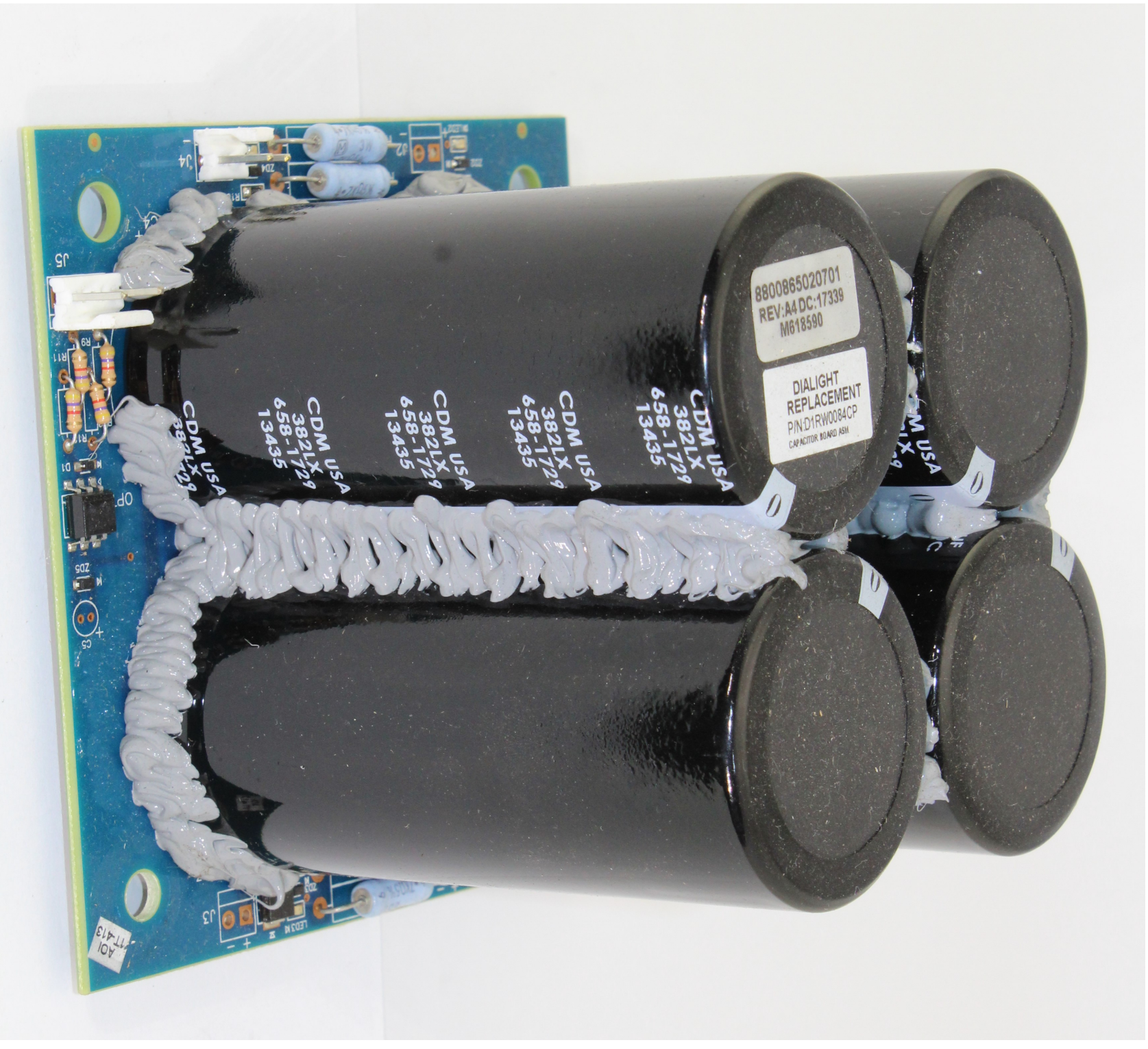
Capacitor PCB, DIRW0084CP, DIR- W008-4CP
